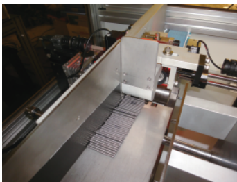
入料倉Unmachined Parts Hopper
